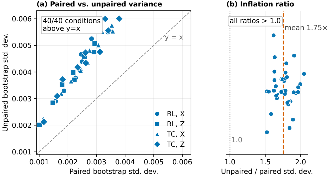
Figure 2: Pairing reduces estimator variance for the decoder-pathway intervention. Panel (a) compares paired and unpaired bootstrap standard deviations for the 40 main conditions; every point lies above the y = x reference line, meaning the unpaired estimator has larger uncertainty. Panel (b) shows the inflation ratio, with mean unpaired/paired standard-deviation inflation of 1.75\times and range 1.52\times – 2.05\times . The semantic cost of discarding pairing—losing rescued/induced transition semantics—is equally fundamental and cannot be recovered by larger sample sizes.
