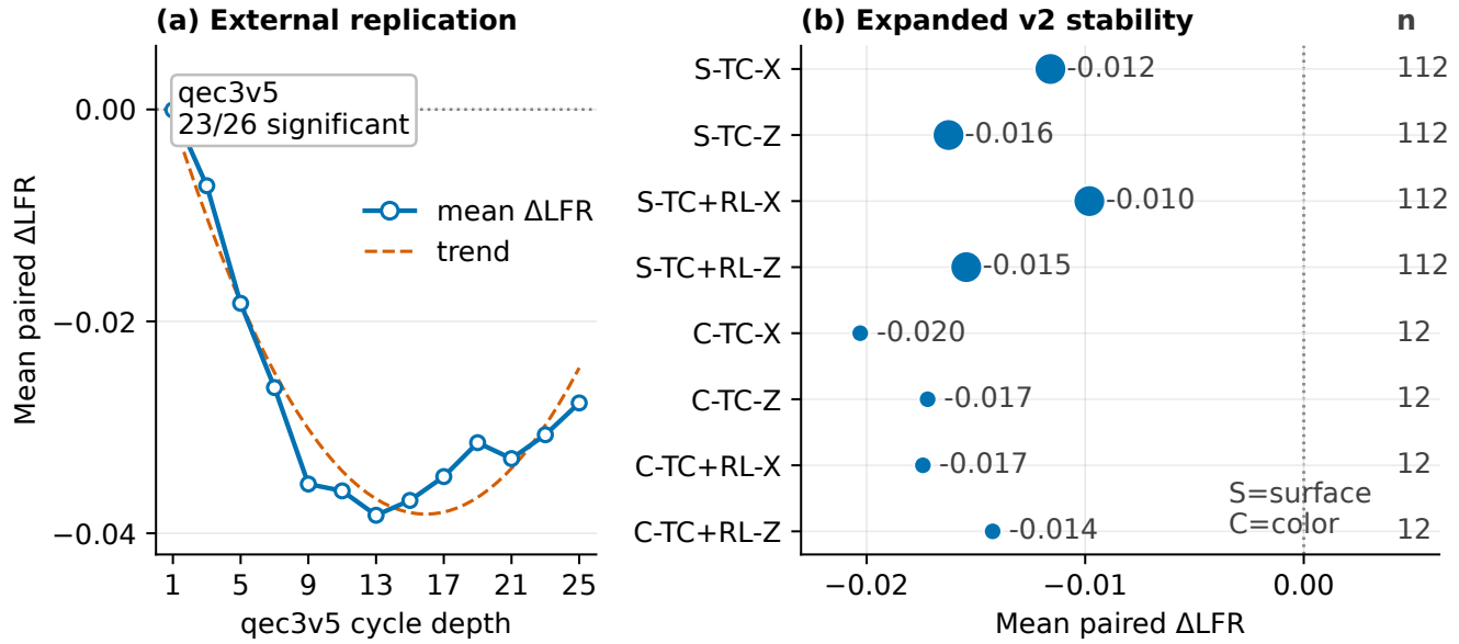
Figure 4: Replication and subgroup stability. Panel (a) aggregates the external qec3v5 replication by cycle depth and shows mean paired \Delta\text{LFR} with a trend line; 23 of 26 qec3v5 conditions are Holm-significant. Panel (b) summarizes the expanded Google RL QEC v2 corpus by code family (S = surface, C = color), control mode, and logical basis. All v2 subgroups have negative mean paired \Delta\text{LFR} , with no subgroup reversal. Across all 496 v2 conditions, the overall mean paired \Delta\text{LFR} is -0.0137 .
