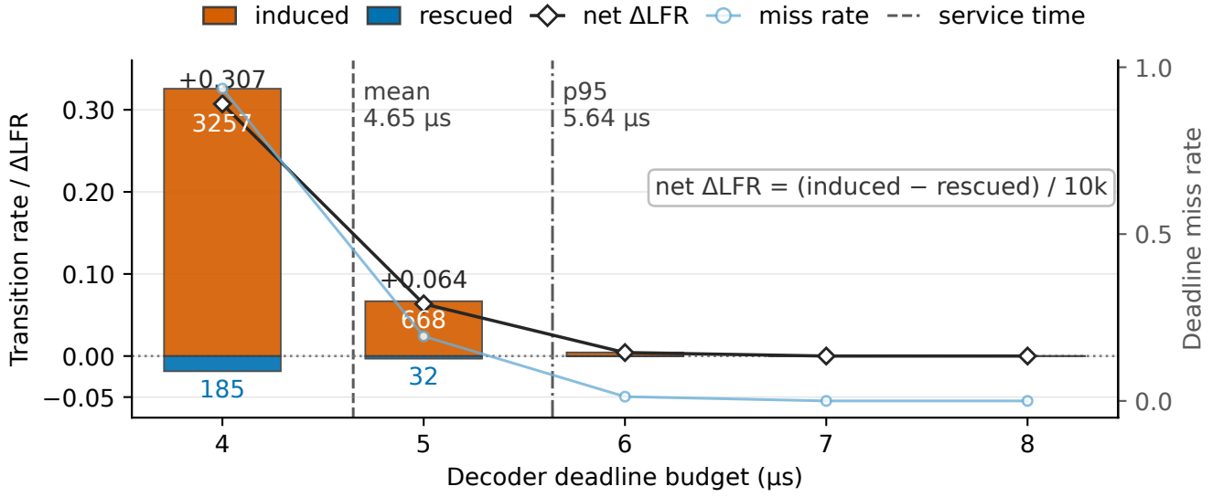
Figure 3: Runtime deadline replay as a paired intervention. Bars decompose the paired transition components: induced failures are plotted upward and rescued failures downward, both normalized by 10,000 paired shots. The black diamond line is the resulting net paired \Delta\text{LFR} = (I - R)/N . The muted line shows the upstream deadline miss rate, and vertical reference lines mark the measured mean and p95 decoder service times. Tight 4 \mu\text{s} and 5 \mu\text{s} budgets induce large failure degradation; the effect collapses by 6–7 \mu\text{s} as the miss rate approaches zero.
