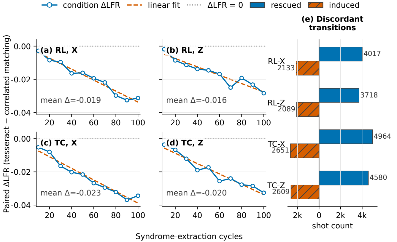
Figure 1: Main decoder-pathway intervention on 40 real Google RL QEC conditions. Each point is the paired \Delta\text{LFR} from replaying the same 10,000 shot records under correlated matching and tesseract, both using SI1000 priors. The four left panels show condition-level trends by control mode and logical basis; the right panel decomposes discordant paired transitions into rescued and induced failures. All 40 conditions are net-rescuing, with 17,279 rescued versus 9,482 induced transitions overall and mean paired \Delta\text{LFR} = -0.0195 .
