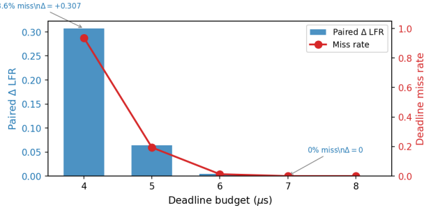
Figure 3. Paired delta LFR (bars) and deadline miss rate (line) as a function of decoder deadline budget. A sharp threshold appears between 4 \mu s and 6 \mu s, corresponding to the region around the measured mean service time of 4.65 \mu s.
