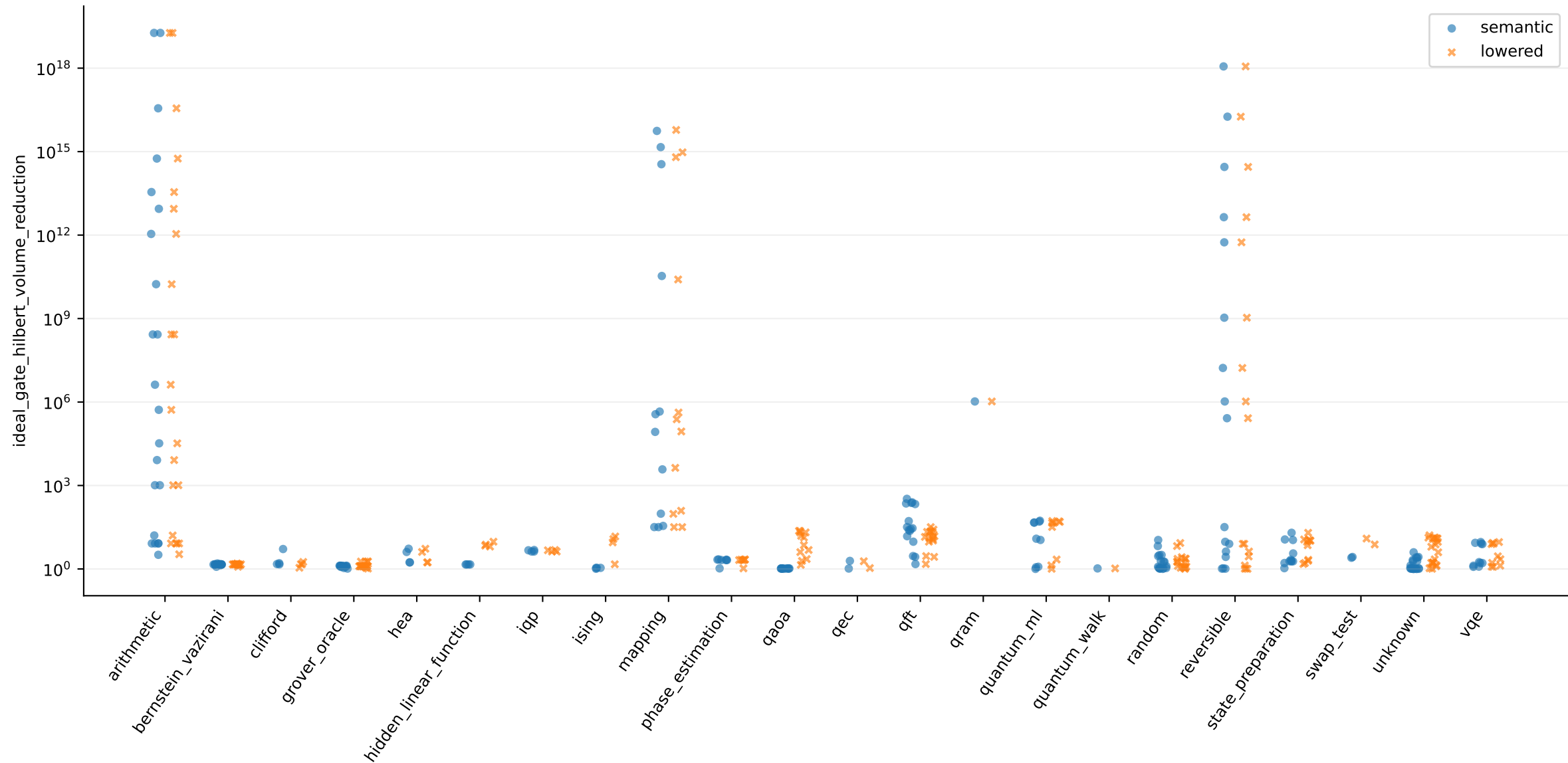
Figure 3 — Every external circuit, n \leq 64 | includes basis-only circuits; no synthetic/generated
