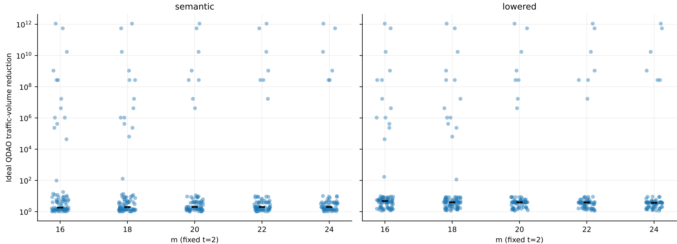
Figure 6 — Static oracle — excludes materialization overhead External 20–40 qubits; each point one circuit/m; black marker median
