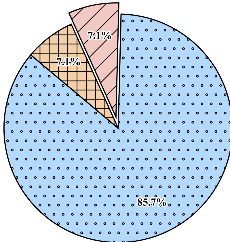
Ours (WorldMind)
