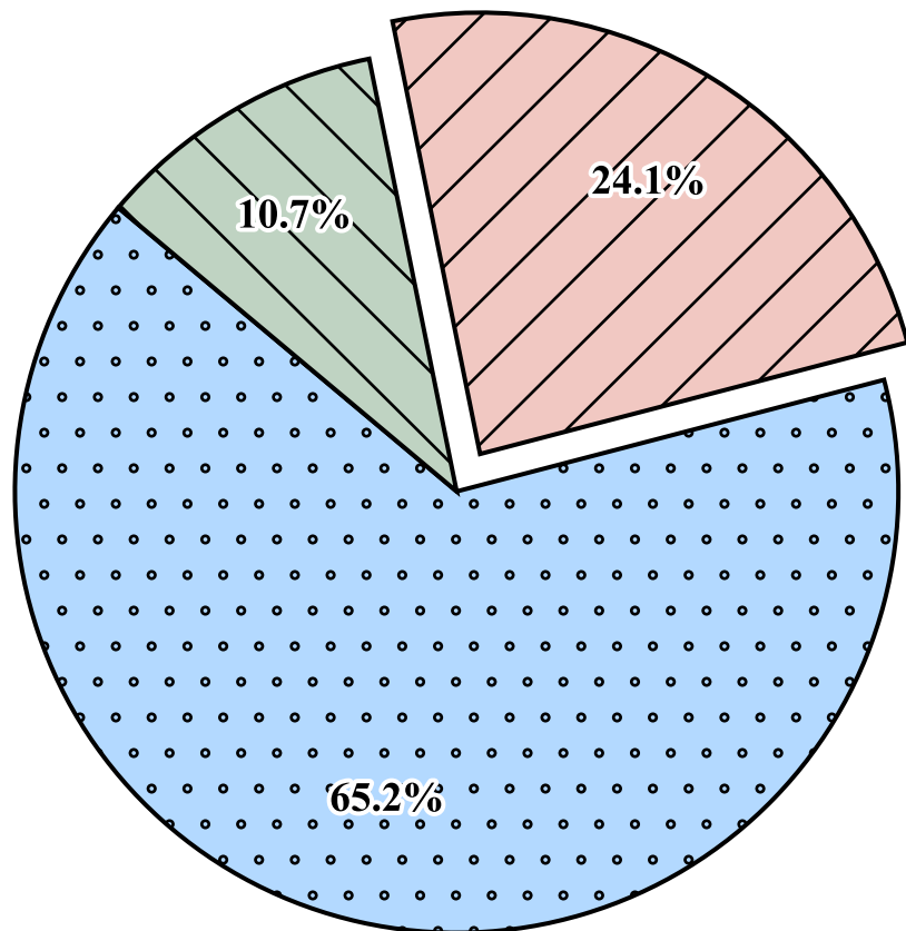
Baseline (ReAct)
