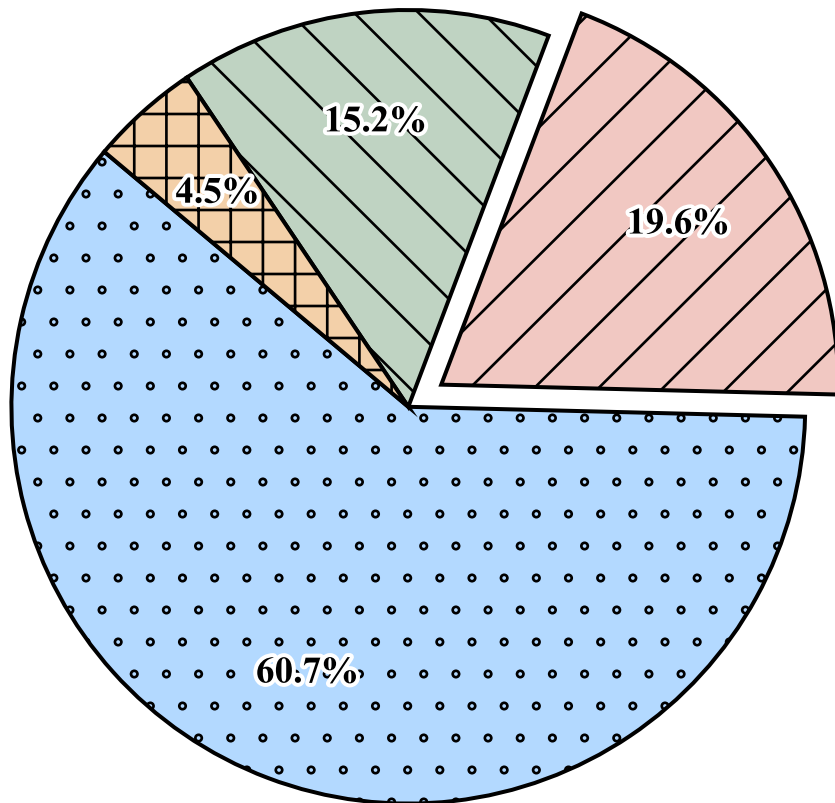
Baseline (ReAct)
