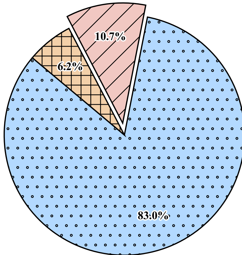
Ours (WorldMind)
