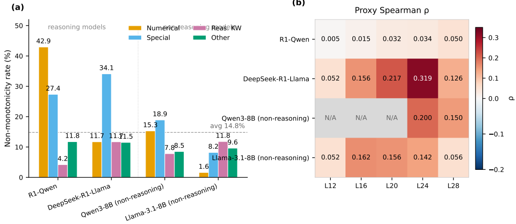
Figure 3: Left: Non-monotonic convergence rates by token role across the 2 \times 2 design (R1-Qwen3-8B, R1-Llama-8B, Qwen3-8B, Llama-3.1-8B; 500 questions each except Qwen3 n=499 ). Right: Cosine-similarity proxy Spearman \rho heatmap. R1-Llama’s moderate \rho=0.32 masks a per-type inversion ( \rho=-0.51 for reasoning keywords).
