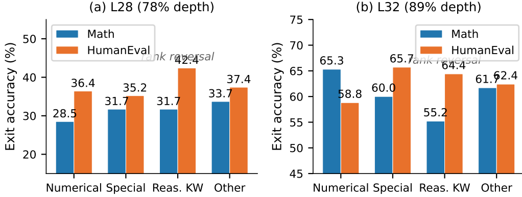
Figure 7: OOD generalization to HumanEval code reasoning. Left (a) : Per-type exit accuracy at L28 (78% depth). Right (b) : Per-type exit accuracy at L32 (89% depth). Ranking reversals between Math and HumanEval are annotated. Overall accuracy closely mirrors math results (+1.4pp at L32).
