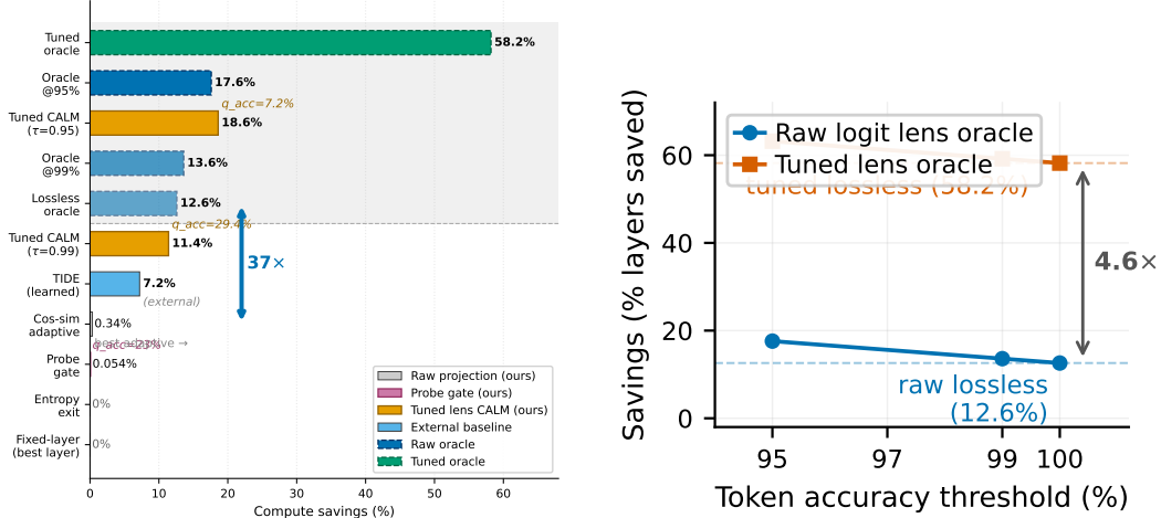
(a) Raw vs. tuned oracle gap (+45.6pp). (b) Oracle savings vs. token acc. Tuned lens: Figure 4: End-to-end exit analysis on R1-Qwen3-8B (300q) → 58.2% Q_Acc at 20.2% savings (5-fold stratified CV; Appendix P); net savings after probe overhead remain ~19.2% (Appendix T.1). Margin and top- k mass drive exit decisions ( |\text{coef}| > 0.5 ), while type identity contributes minimally ( |\text{coef}| < 0.02 ; per-type gates: V2c 64%, 18.1% savings). Compound error remains the binding constraint: 68.2% vs. \approx 91\% near-full-depth Q_Acc.
