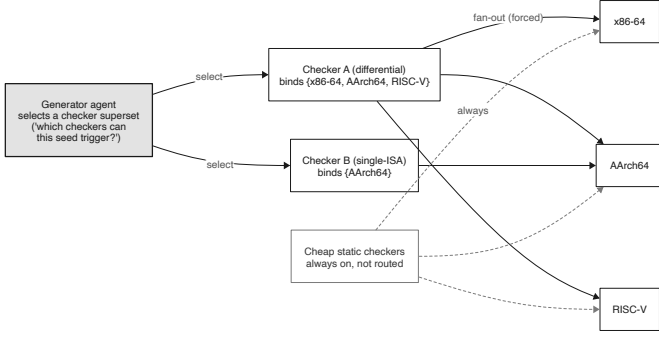
Fig. 11. Checker-bound ISA routing: the agent selects checkers; each checker fans out to its bound ISAs; cheap checkers always on.
