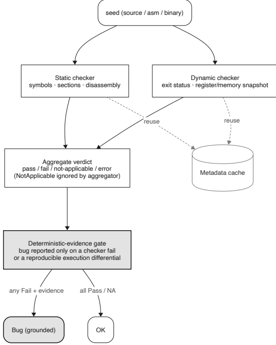
Fig. 9. Invariant \rightarrow verdict flow: four-state checkers, NotApplicable transparency, and a deterministic-evidence gate before any bug is reported.
