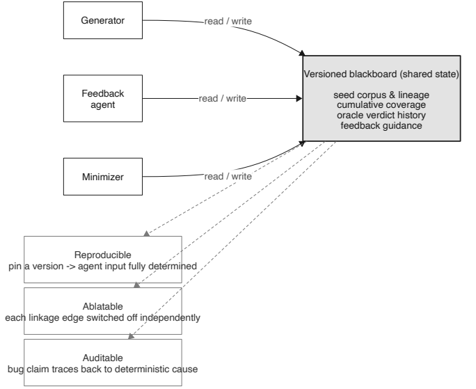
Fig. 10. The blackboard: all inter-agent linkage flows through versioned shared state, enabling reproduce / ablate / audit.
