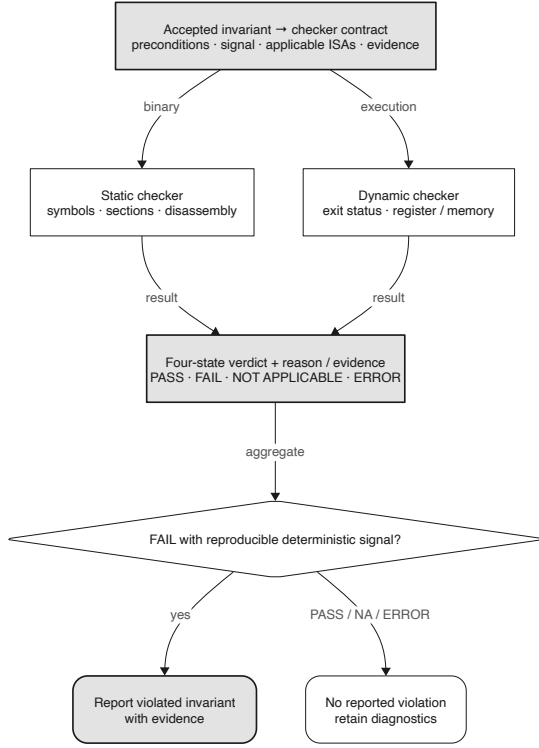
Fig. 10. An accepted invariant is translated into a static or dynamic checker; four-state verdicts pass through a deterministic-evidence gate before any finding is confirmed.
