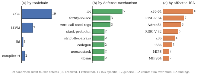
Fig. 12. Silent-failure defects found by DeFuzz across 29 confirmed findings: (a) by producing toolchain, (b) by defense mechanism, (c) by affected ISA. ISA counts sum over multi-ISA findings.
