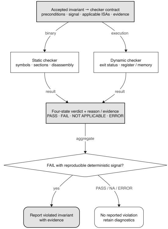
Fig. 10. An accepted invariant is translated into a static or dynamic checker; four-state verdicts pass through a deterministic-evidence gate before any finding is confirmed.
