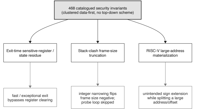
Fig. 7. Bottom-up root-cause families over 468 invariants; three families recur across mechanism and ISA.
