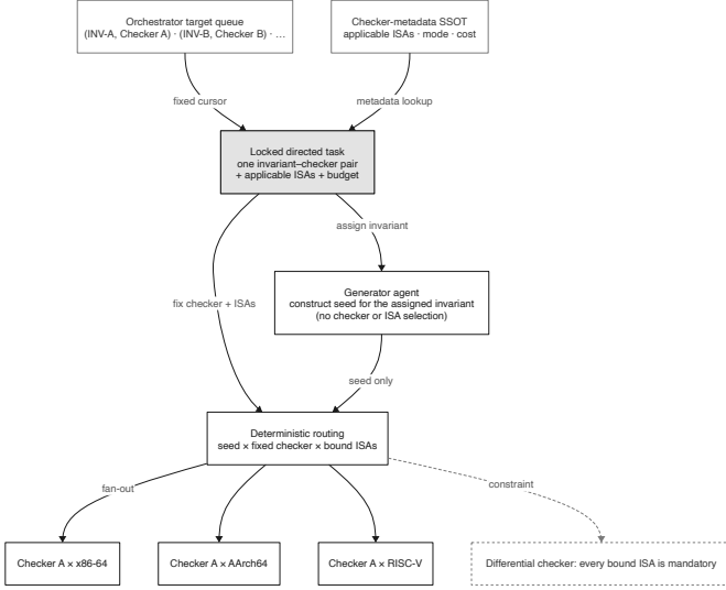
Fig. 12. Deterministic target scheduling: one invariant-checker pair remains fixed for its budget, while checker metadata expands the applicable ISAs and cheap static checkers remain enabled.
