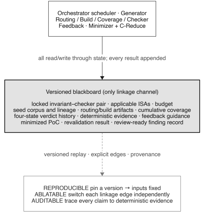
Fig. 11. The blackboard: all inter-agent linkage flows through versioned shared state, enabling reproduce / ablate / audit.
