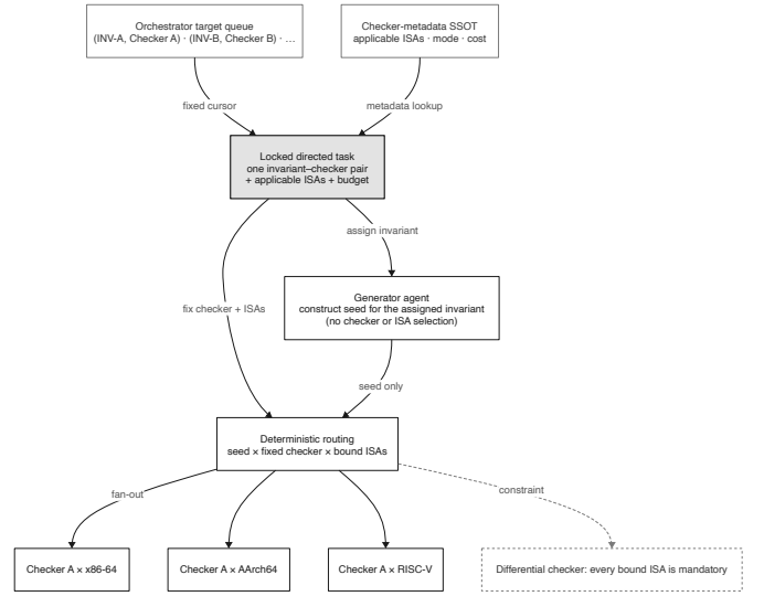
Fig. 12. Deterministic target scheduling: one invariant-checker pair remains fixed for its budget, while checker metadata expands the applicable ISAs and cheap static checkers remain enabled.
