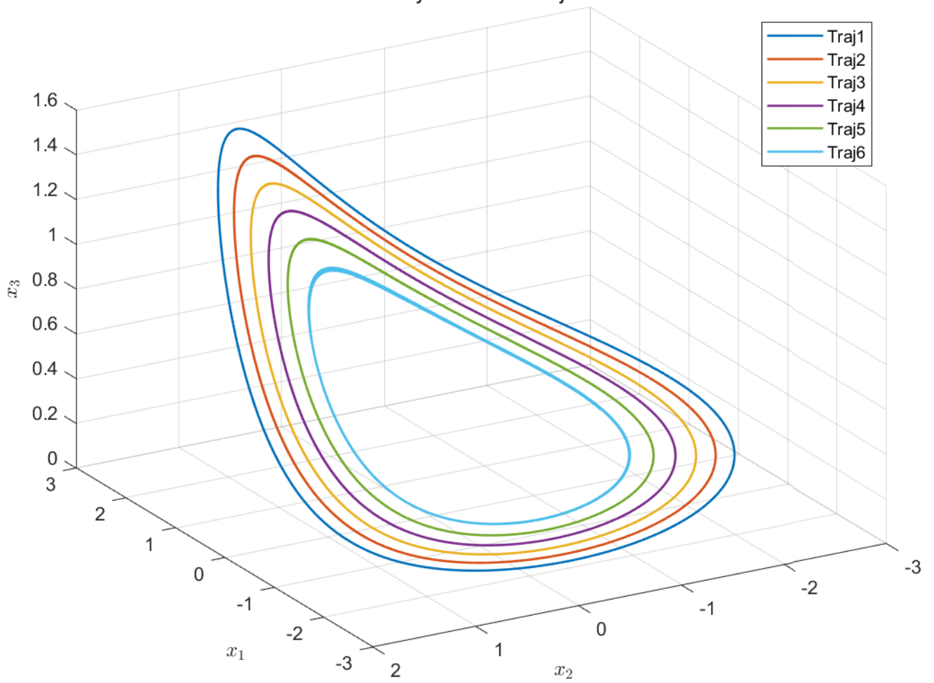
Rossler System State Trajectories
