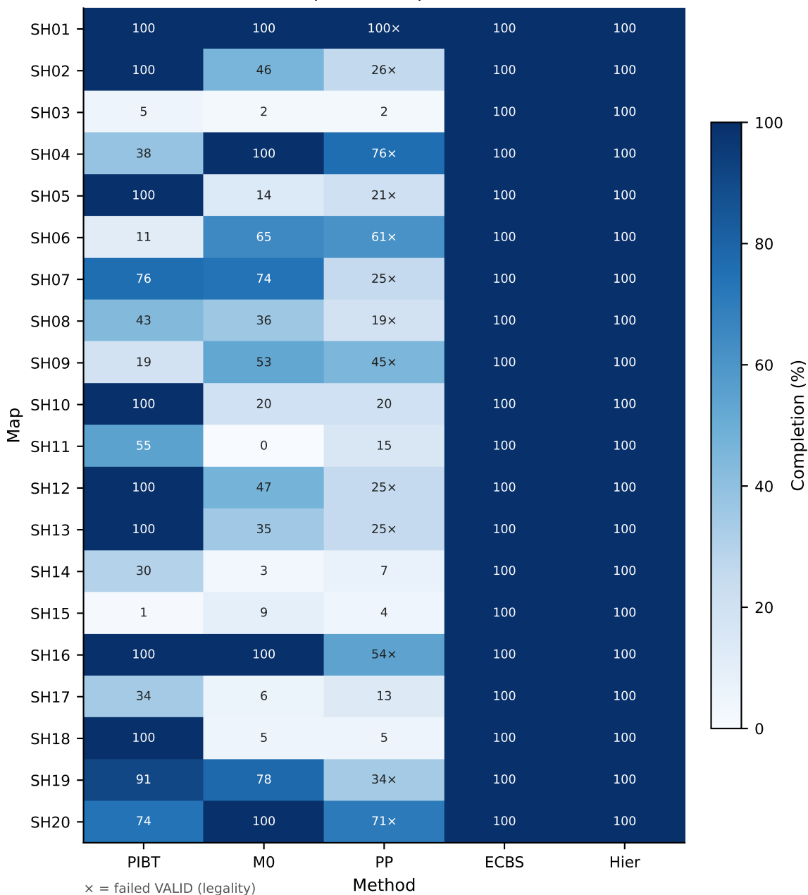
Per-map task completion (%)
