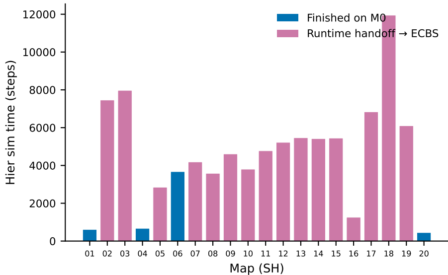
(b) Hier sim time by path
