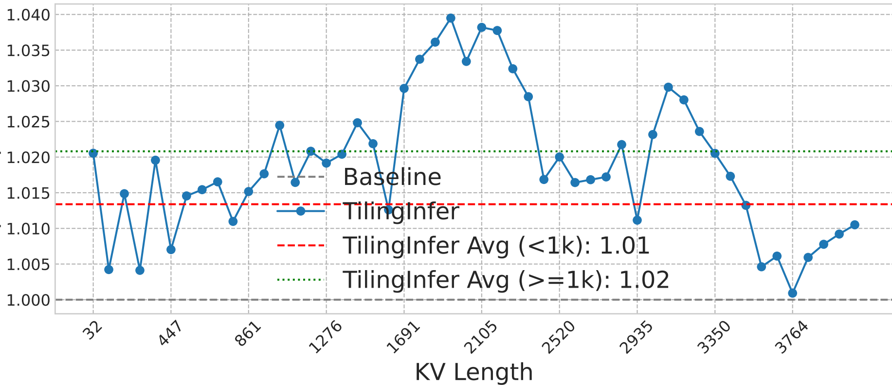
Speedup Ratio
