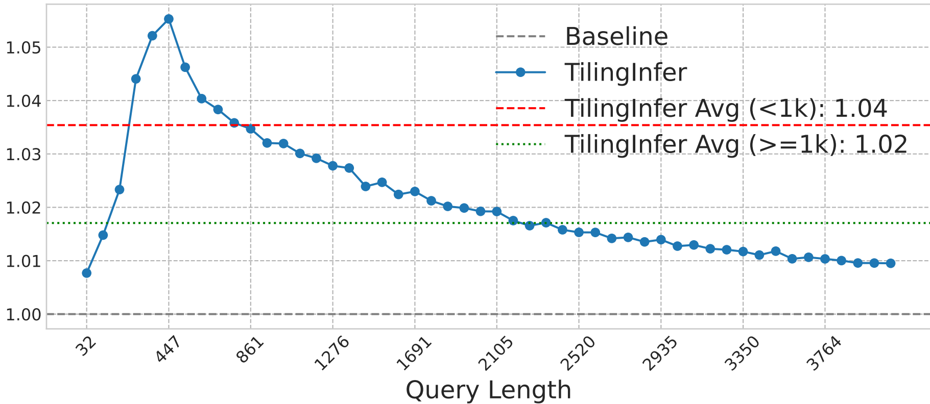
Speedup Ratio
