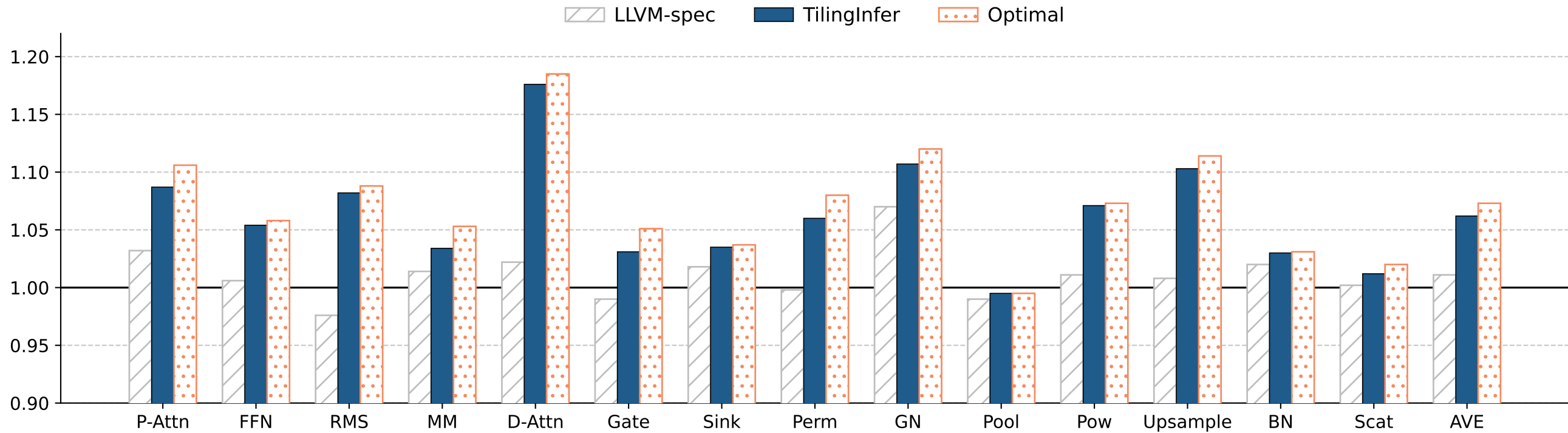
Normalized Speedup
