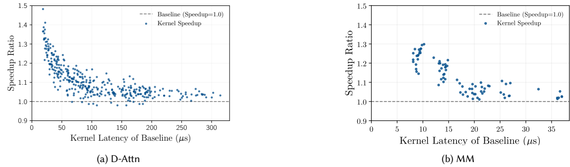
Fig. 13. Kernel speedup versus Baseline device-kernel latency for D-Attn and MM. Blue points report the speedup of TilingInfer relative to Baseline.
