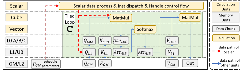
Fig. 3. Execution flow of Flash Attention kernel \text{kernel\_fa} on the Ascend architecture. The Scalar unit acts as the central scheduler. It continuously performs scalar calculations and dispatches instructions based on runtime parameters. The heavy scalar workload required by generic kernels may lead to a scalar bottleneck.
