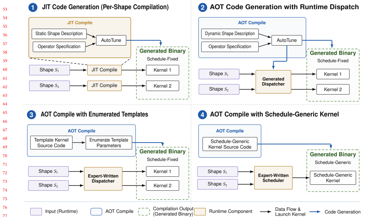
Fig. 1. Four ways to compile and execute dynamic-shape operators.
