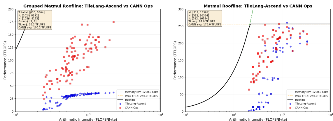
Fig. 1. Ascend roofline comparison of the starting implementations used to assess baseline comparability: Grouped Matmul (left) and Matmul (right). These response-only plots characterize CANN and TileLang-Ascend, not TilingInfer.
