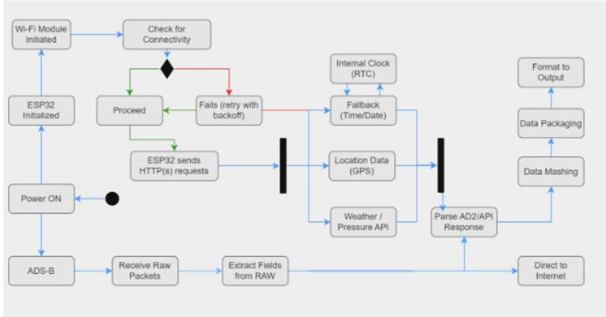
Figure 4.4.1: Communications Subsystem Block Diagram
