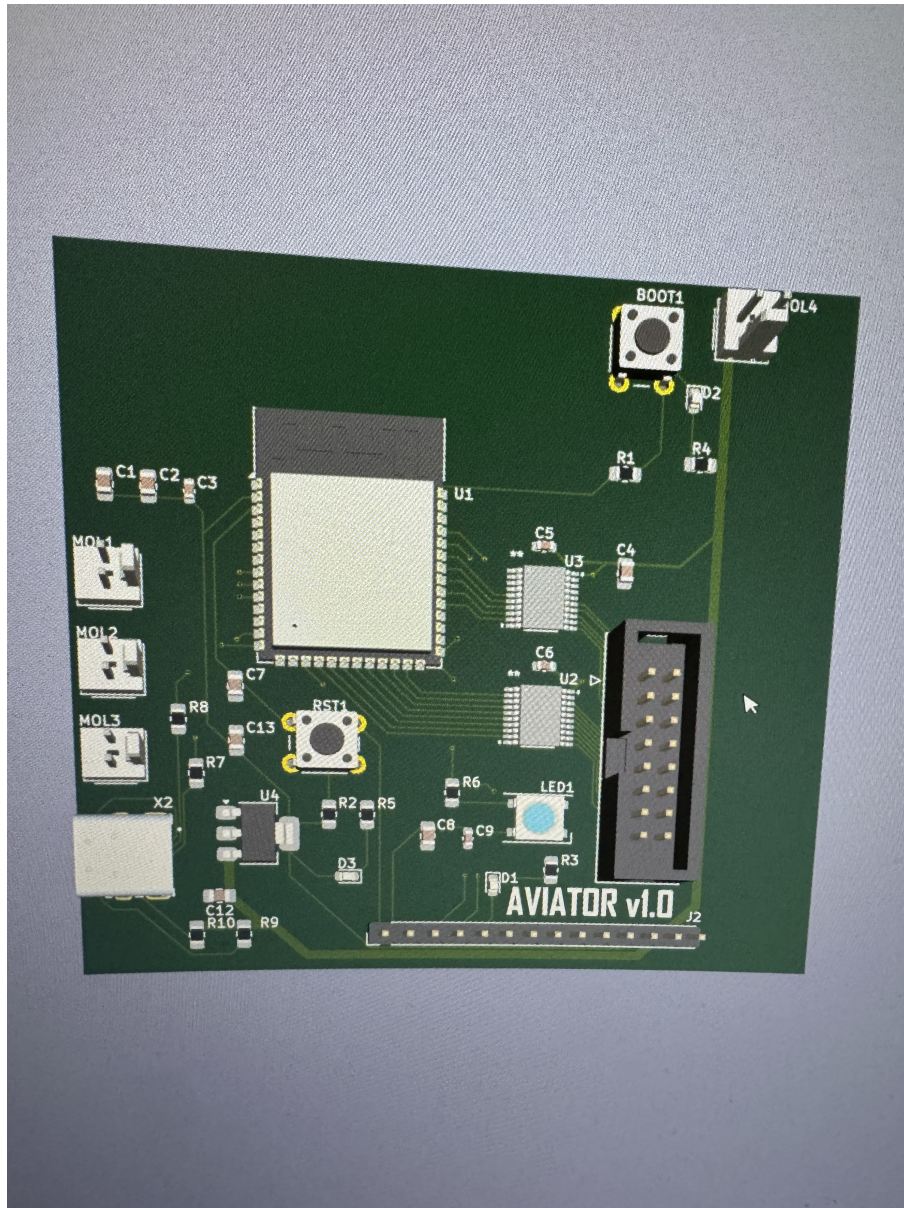
Figure 5.2.2: PCB CAD Layout
