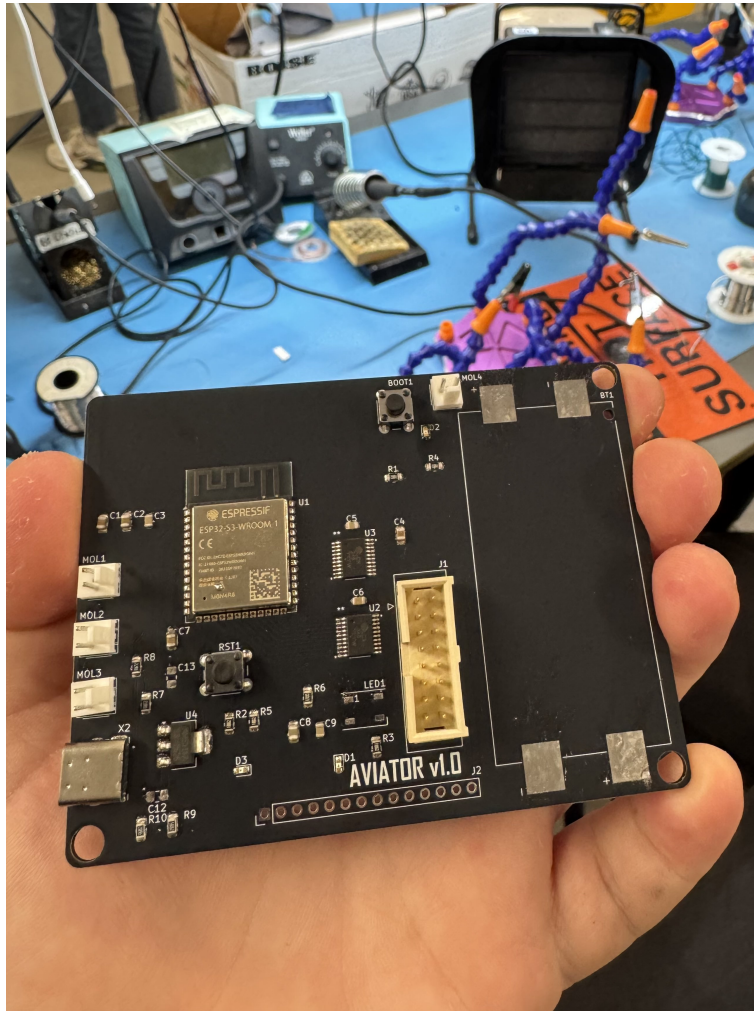
Figure 3.5.2: Photograph of assembled PCB
