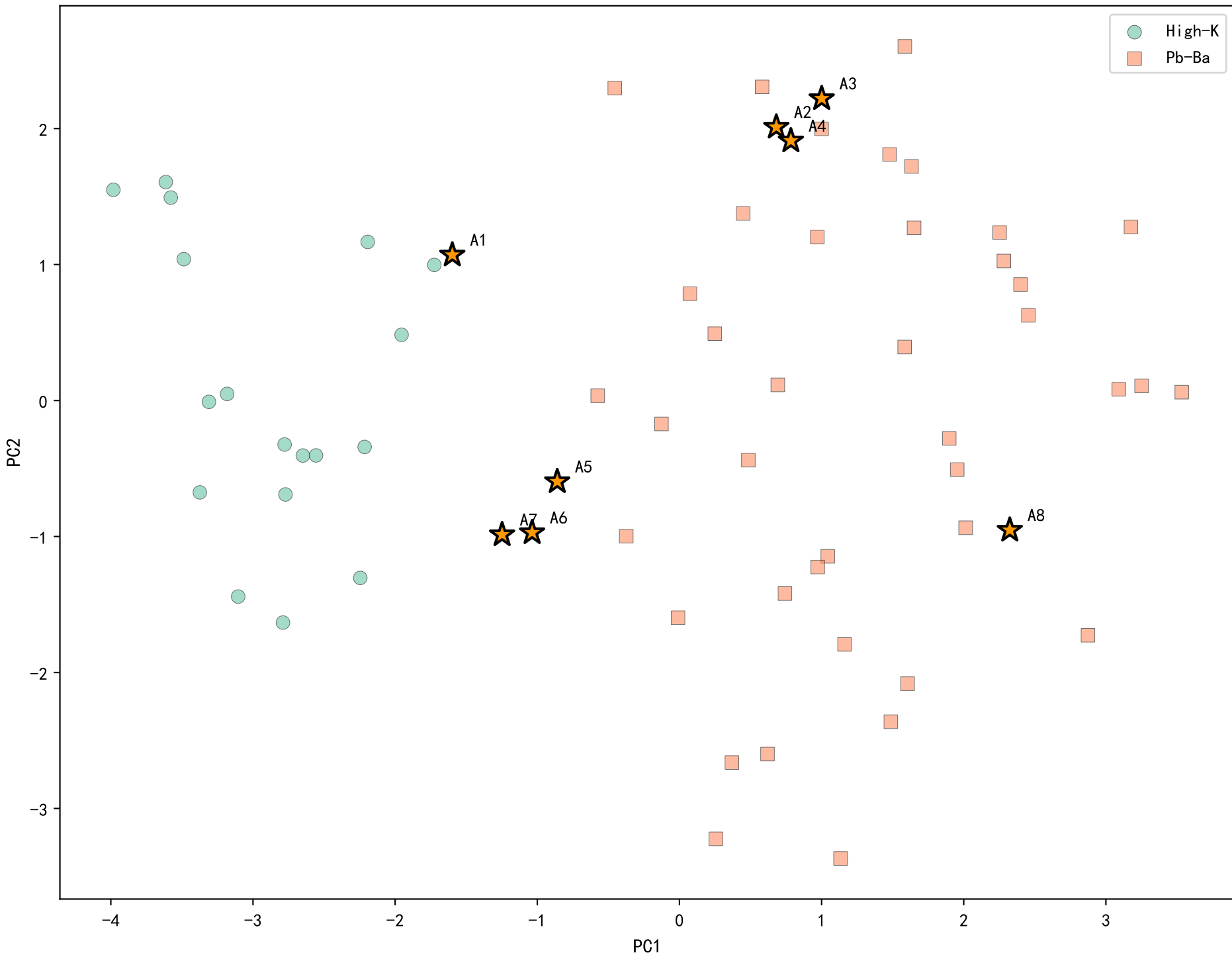
PCA Projection: Training Data + Unknowns (35.9% + 17.5% variance)
