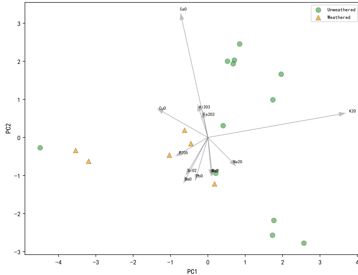
High-K Glass (PC1=33.8%, PC2=22.5%)
