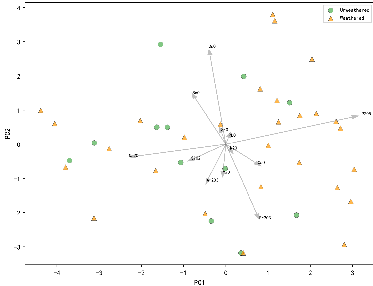
Pb-Ba Glass (PC1=38.1%, PC2=23.6%)
