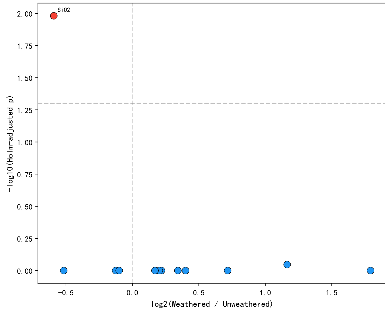
Pb-Ba Glass: Weathering Effect
