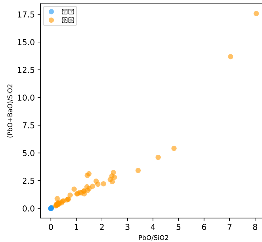
Q2a: Key Ratio Scatter Matrix
