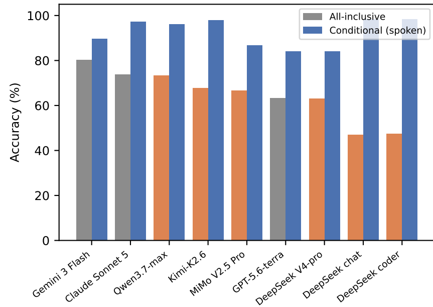
(a) Nine models, identical 500-variant subset
