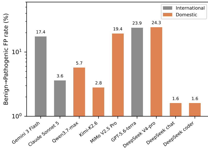
(b) False-positive rate (log scale)
