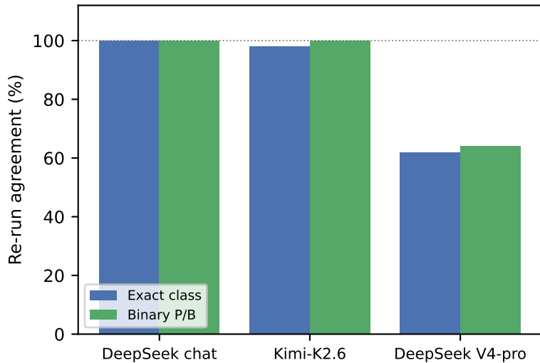
(a) Output determinism (temp=0, n=50)
