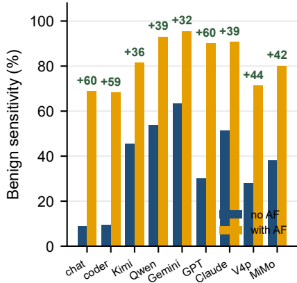
A AF ablation (9 models, n = 356 Benign)
