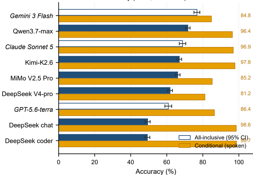
A Dual-metric accuracy (n = 2,555/model)
