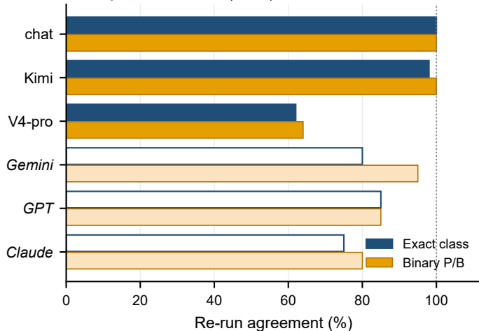
A Output determinism (T = 0)
