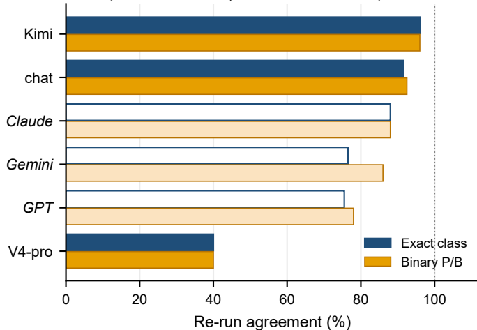
A Output determinism ( T = 0 , n = 200/\text{model} )
