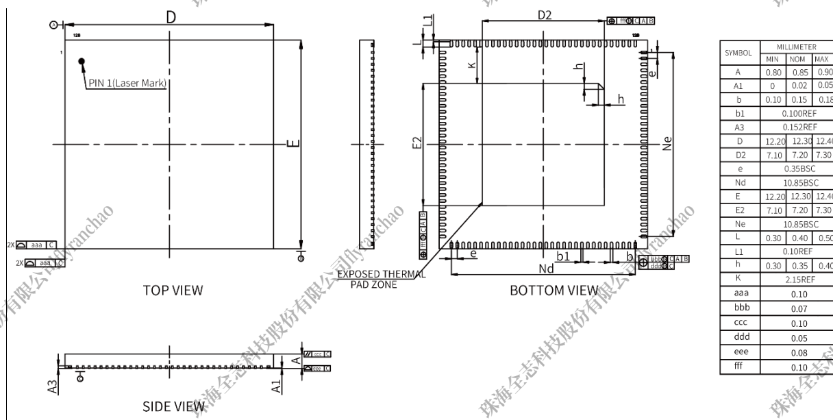
Figure 6-2 Package Dimension
