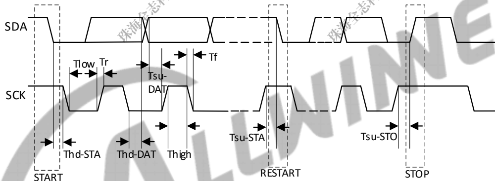
Figure 4-21 TWI Timing
