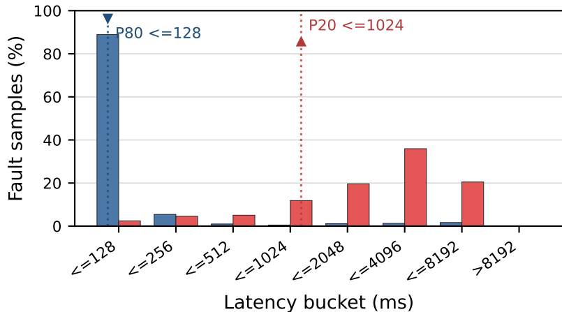
(a) GAPBS BC, window 32 (332s) Local n=8,958 / Remote n=139,334
