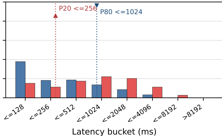
(b) BTree, window 130 (1318s) Local n=169,459 / Remote n=550,088
