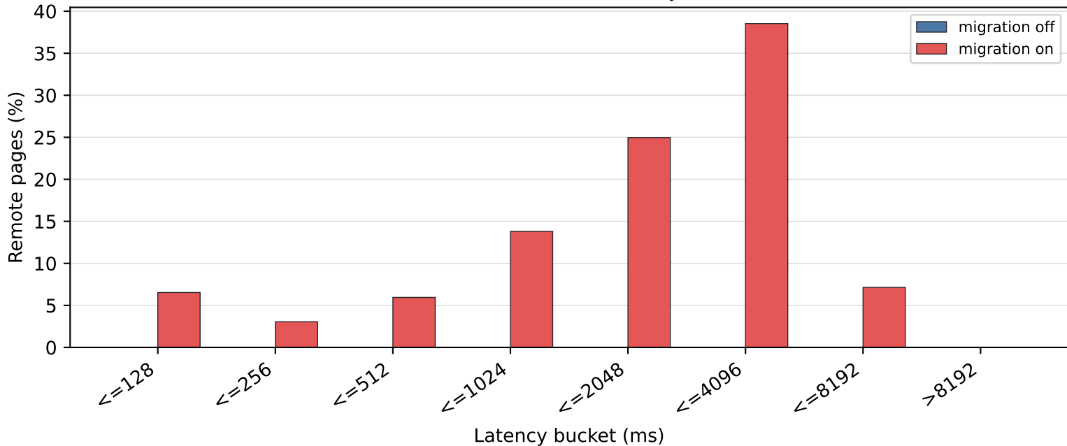
Remote NUMA hint fault latency distribution
