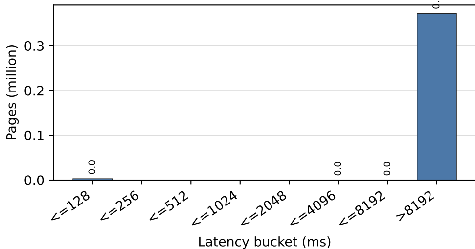
local pages (total=375,506)
