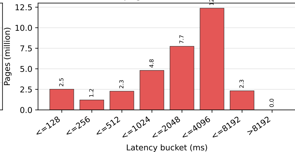
remote pages (total=33,262,100)
