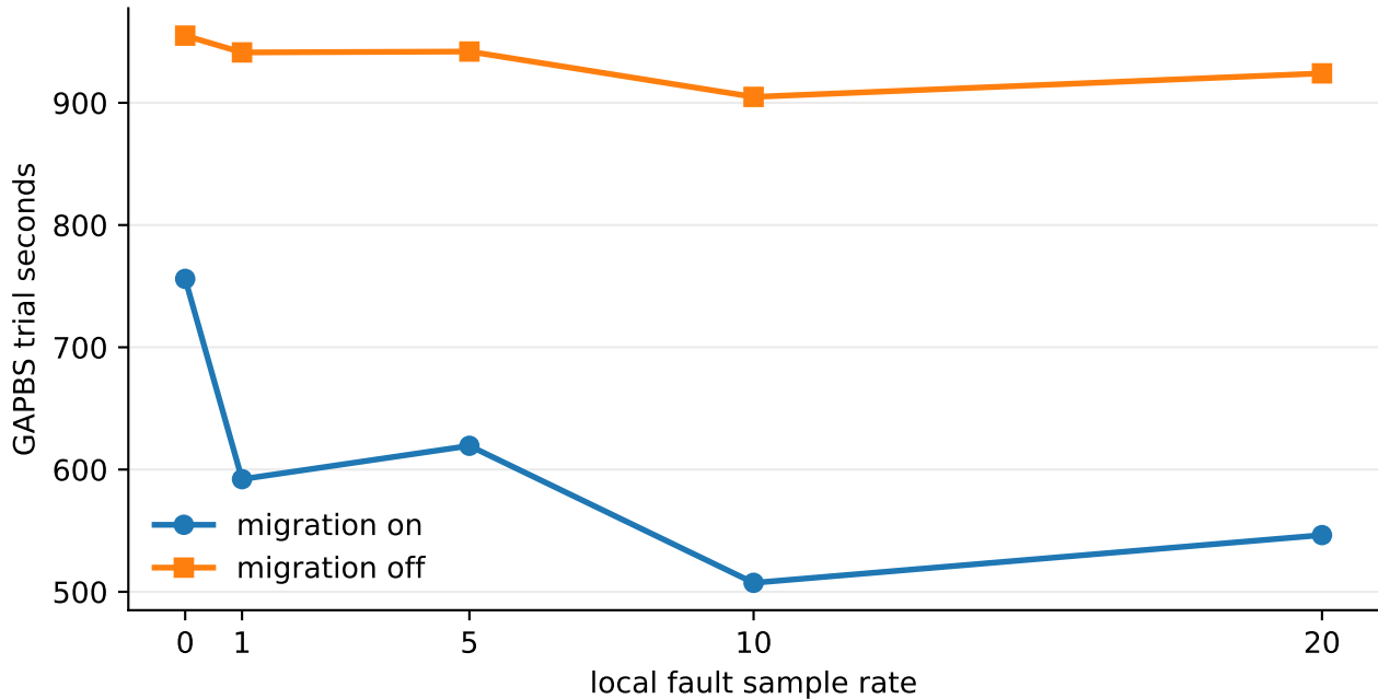
GAPBS BC g29 trial time: migration on vs off
