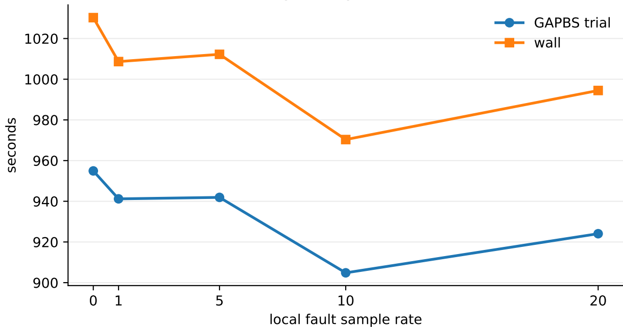
GAPBS BC g29, migration off runtime
