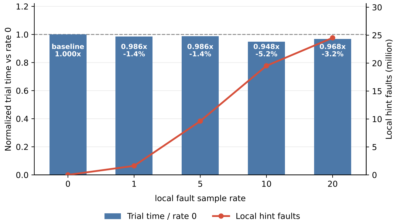
Migration off: runtime vs local hint faults
