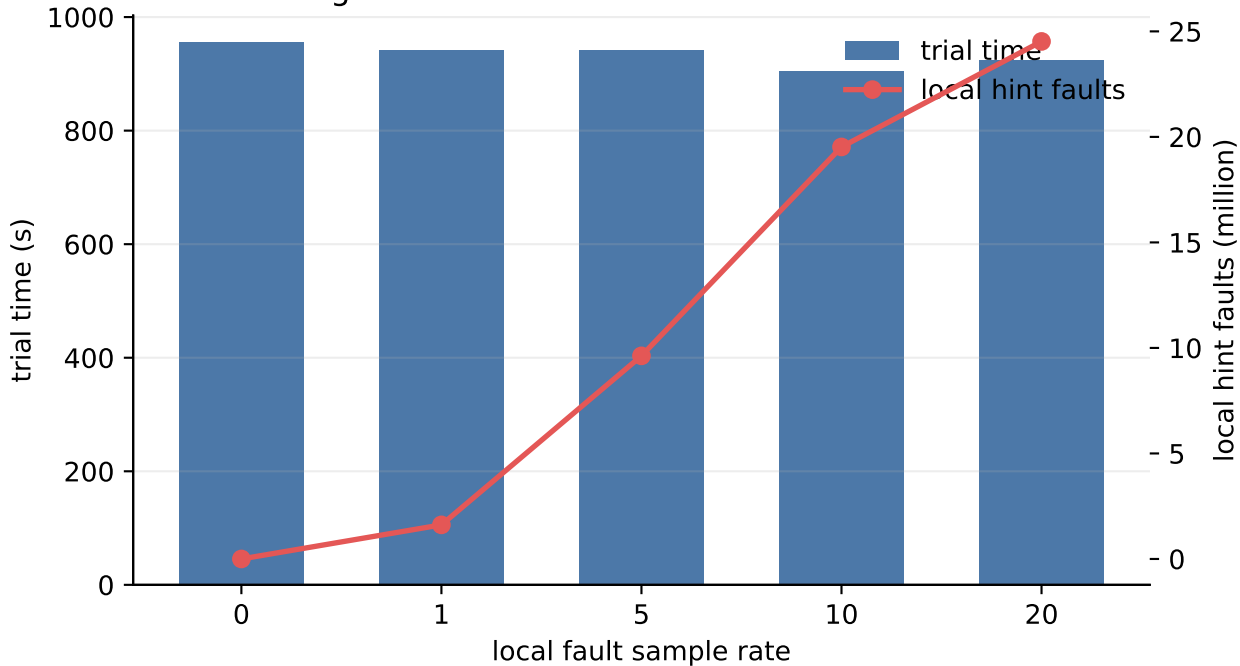
Migration off: trial time and local hint faults
