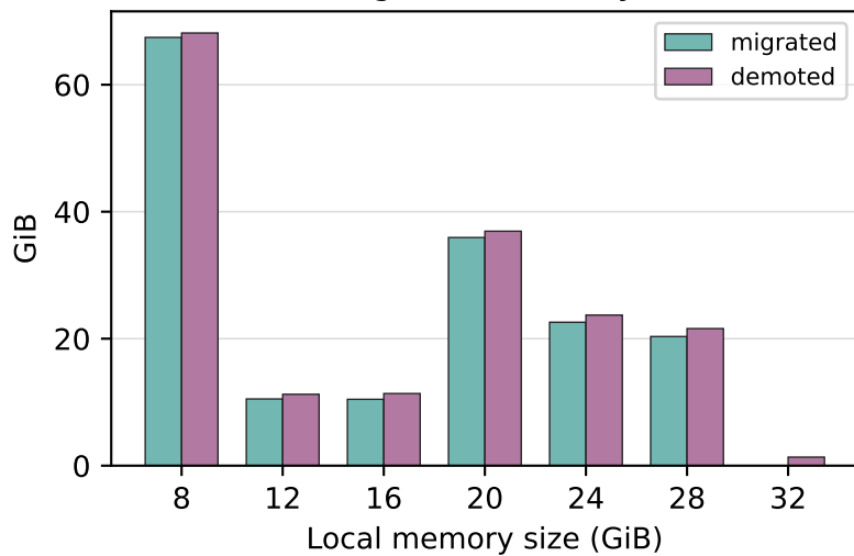
Migration activity
