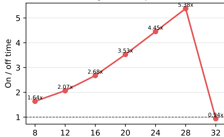
Kernel activity
