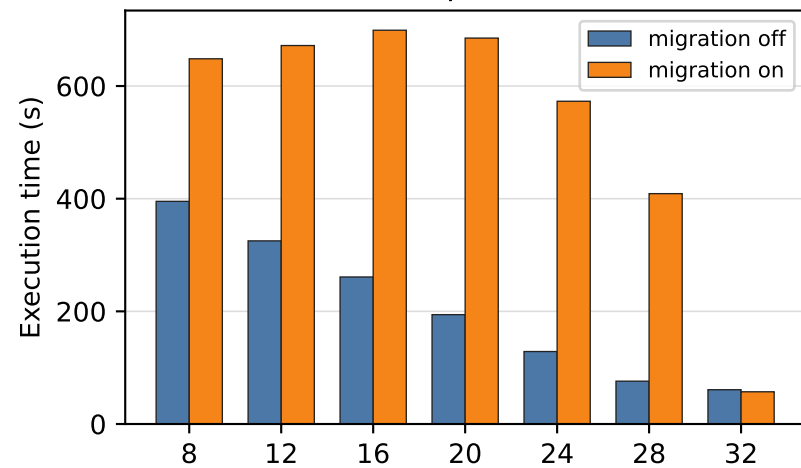
Migration activity
