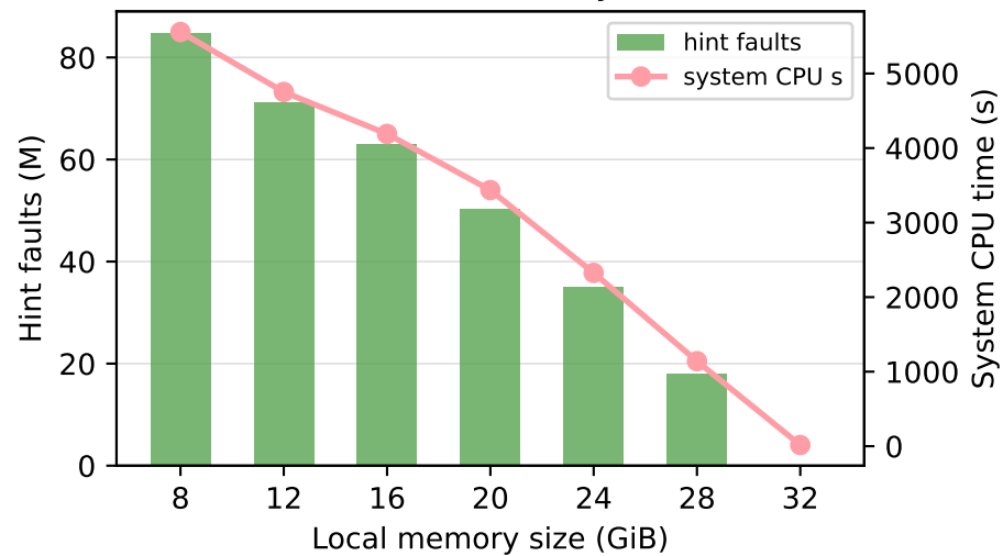
Kernel activity
