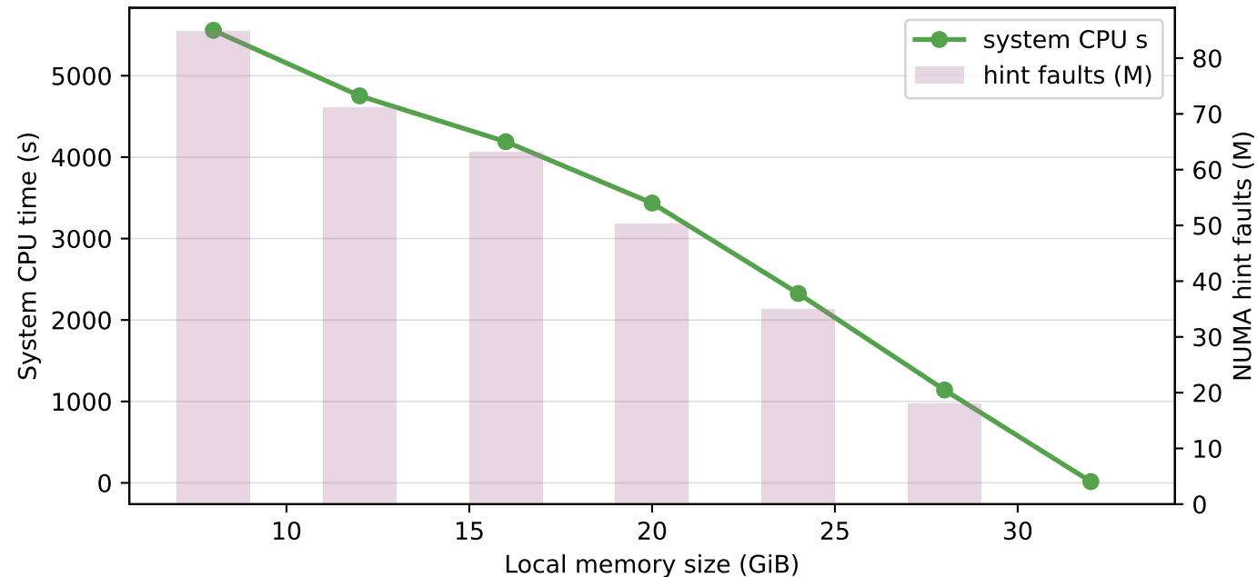
Kernel activity by local memory size
