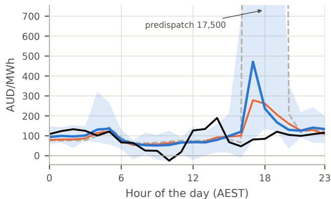
NSW, predispach overstates the peak (24 Oct 2024)
