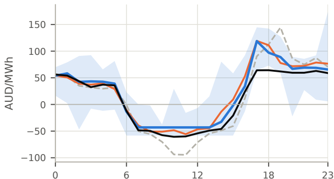
NSW, predispach overstates the peak (24 Oct 2024)
