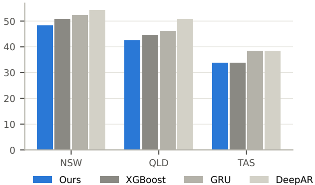
Raw prices: test MAE (AUD/MWh)
