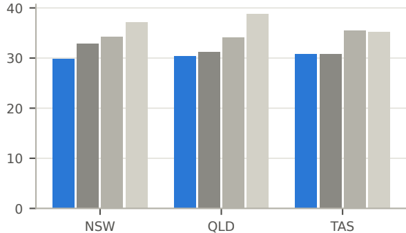
Prices capped at 650 AUD/MWh: test MAE (AUD/MWh)
