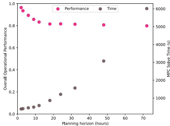
Fig. B.11. Variation of perfect forecast MPC operational performance and computation time with planning horizon, T .
