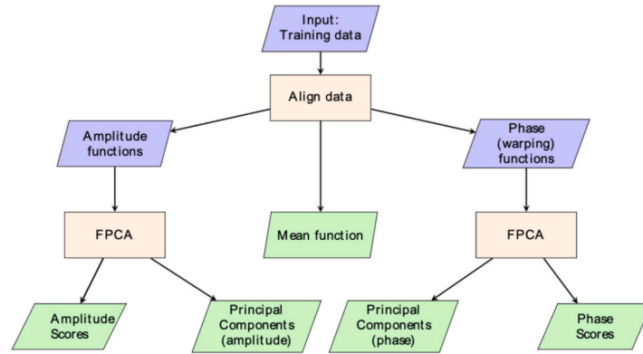
Fig. D.12. Schematic process for functional principal component analysis (fPCA).
