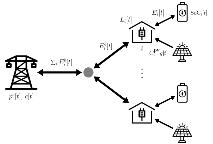
Fig. 1. Energy flow schematic for test multi-building energy system. (Icon credits: Symbolon ).
