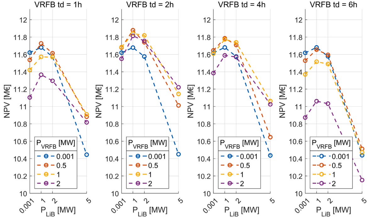
Fig. 5. Net Present Value (NPV) coming from a wind plant ( P_{n,wind} = 10 MW) bidding on DA and aFRR market after the installation of a HESS for different storage sizes, for investment scenario B, assuming a simple battery model.
