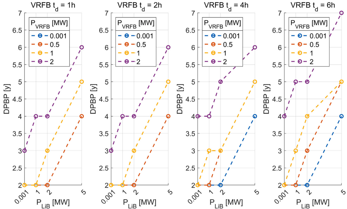
Fig. 4. Discounted Payback Period (DPBP) coming from a wind plant ( P_{n,wind} = 10 MW) bidding on DA and aFRR market after the installation of a HESS for different storage sizes, for investment scenario B.
