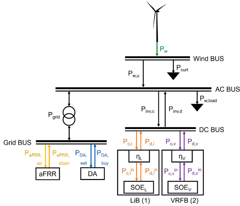
Fig. 1. Scheme of the battery-assisted grid-connected renewable system.
