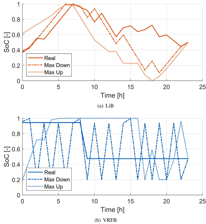
Fig. 6. Example of optimal LiB and VRFB SOC (state of charge) for different scenarios of the robust optimization: realistic, worst-case of maximum up-regulation activation, worst-case of maximum down-regulation activation.
