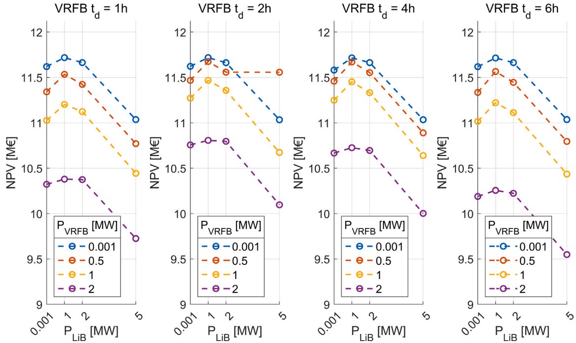
Fig. 3. Net Present Value (NPV) coming from a wind plant ( P_{n,wind} = 10 MW) bidding on DA and aFRR market after the installation of a HESS for different storage sizes, for investment scenario B.
