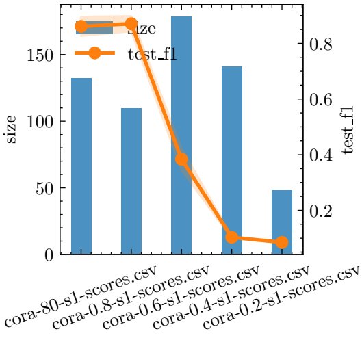
cora rule size
