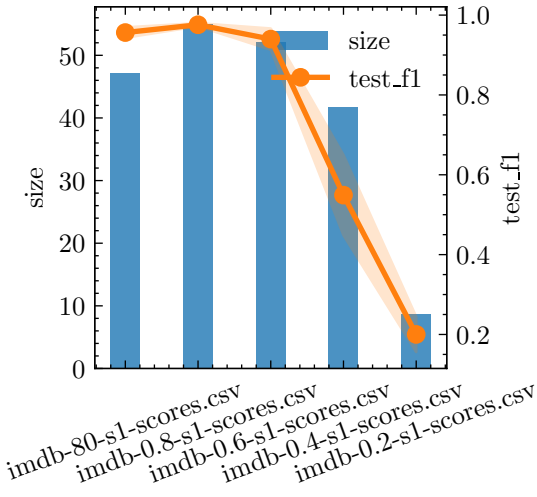
imdb rule size
