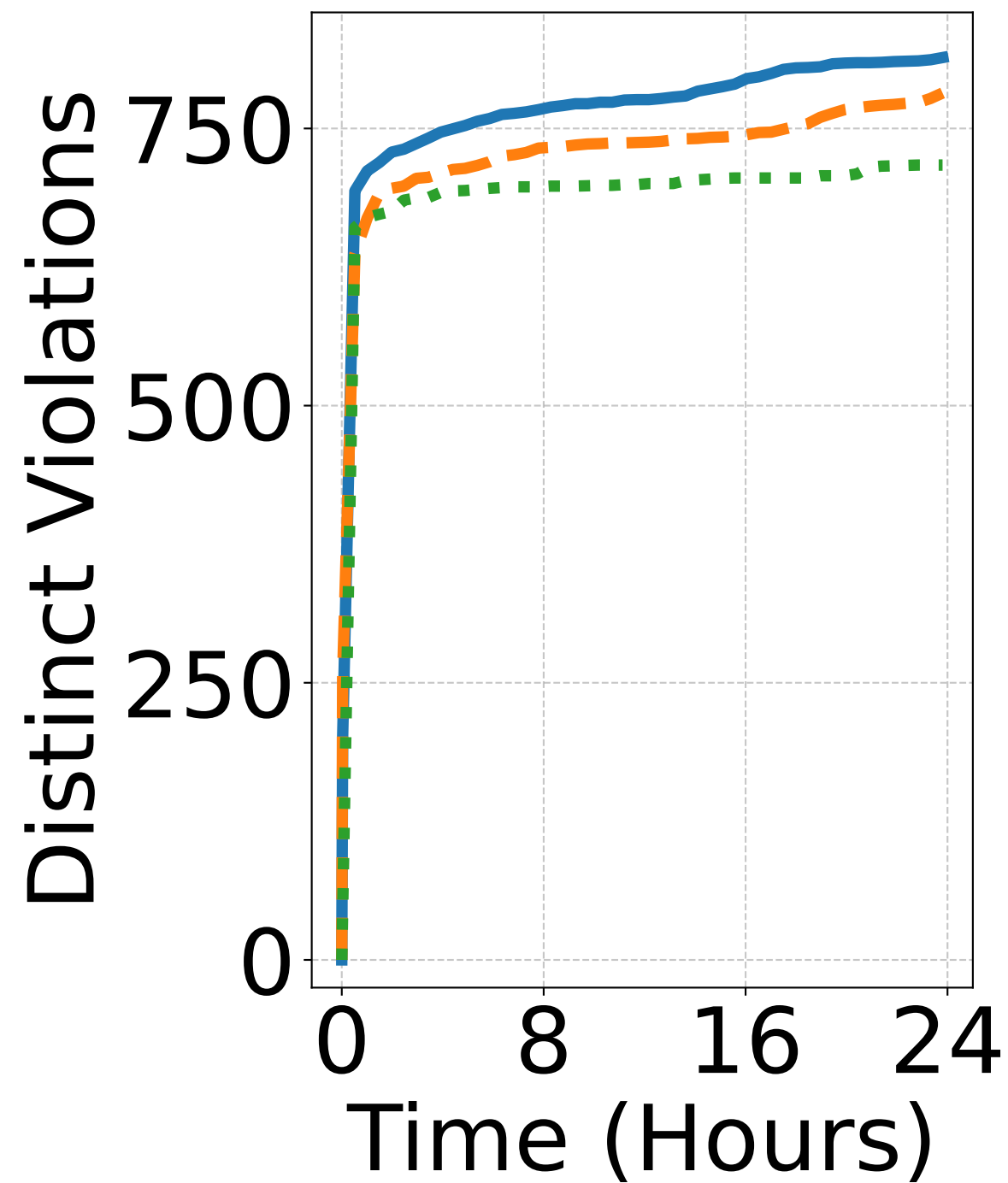
Cassandra
