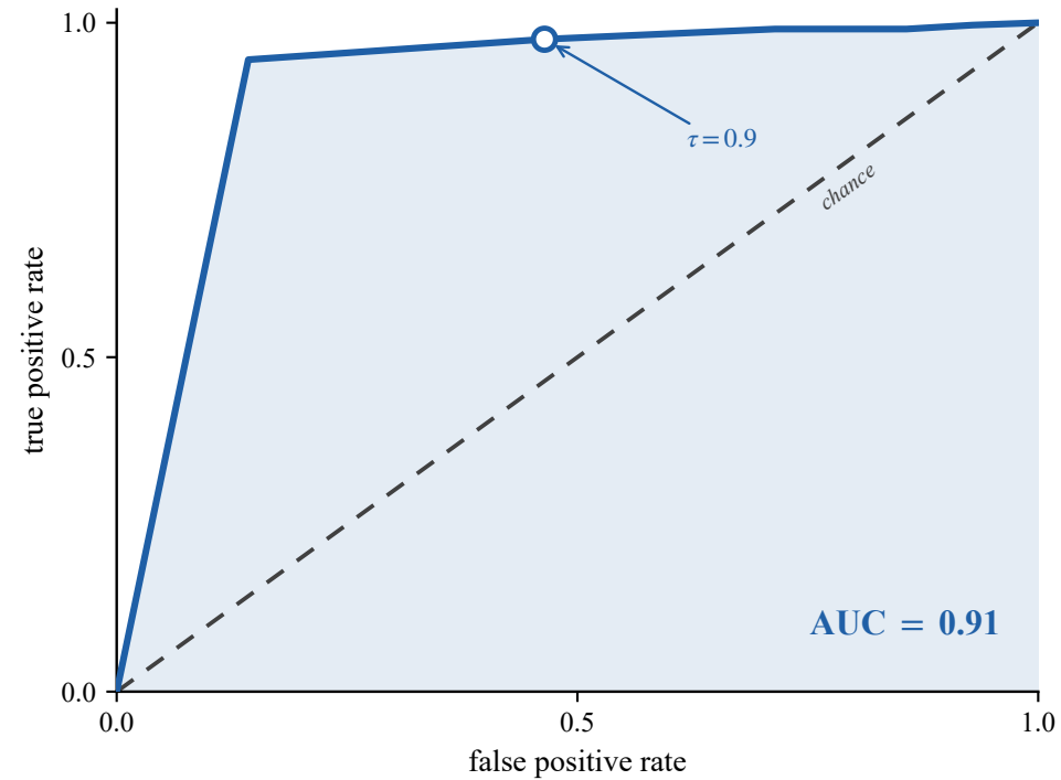
(a) ROC on the external TMM benchmark
