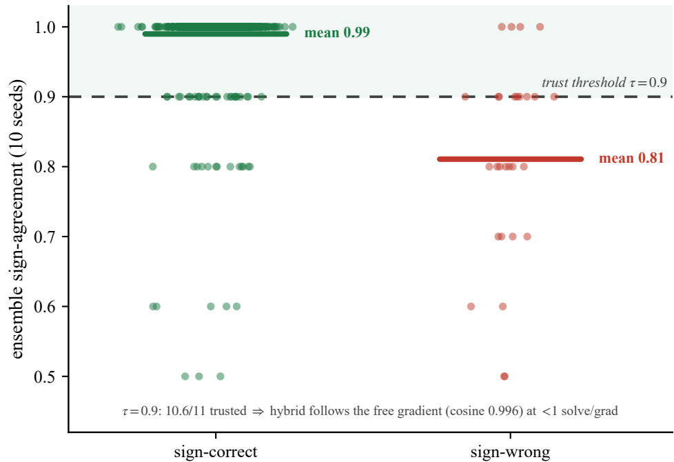
(b) reliable vs. unreliable components
