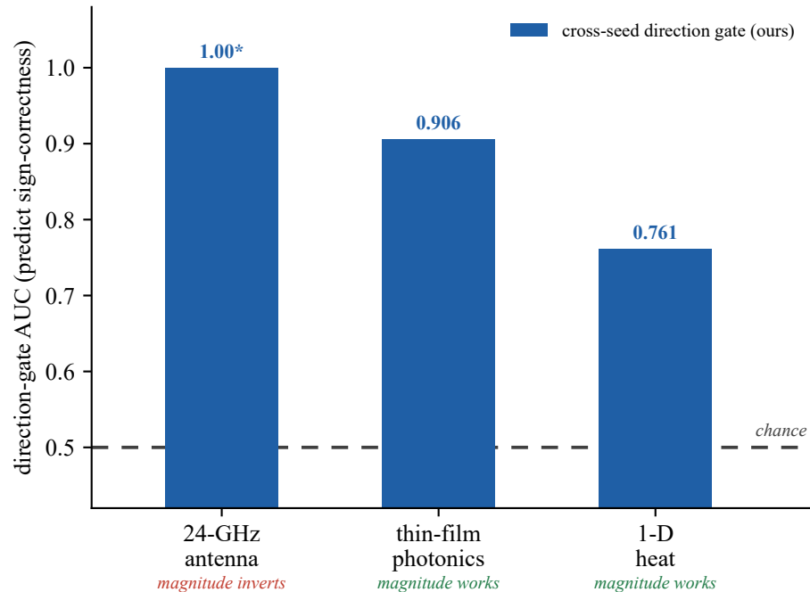
(b) direction: one fixed rule across three physics families
