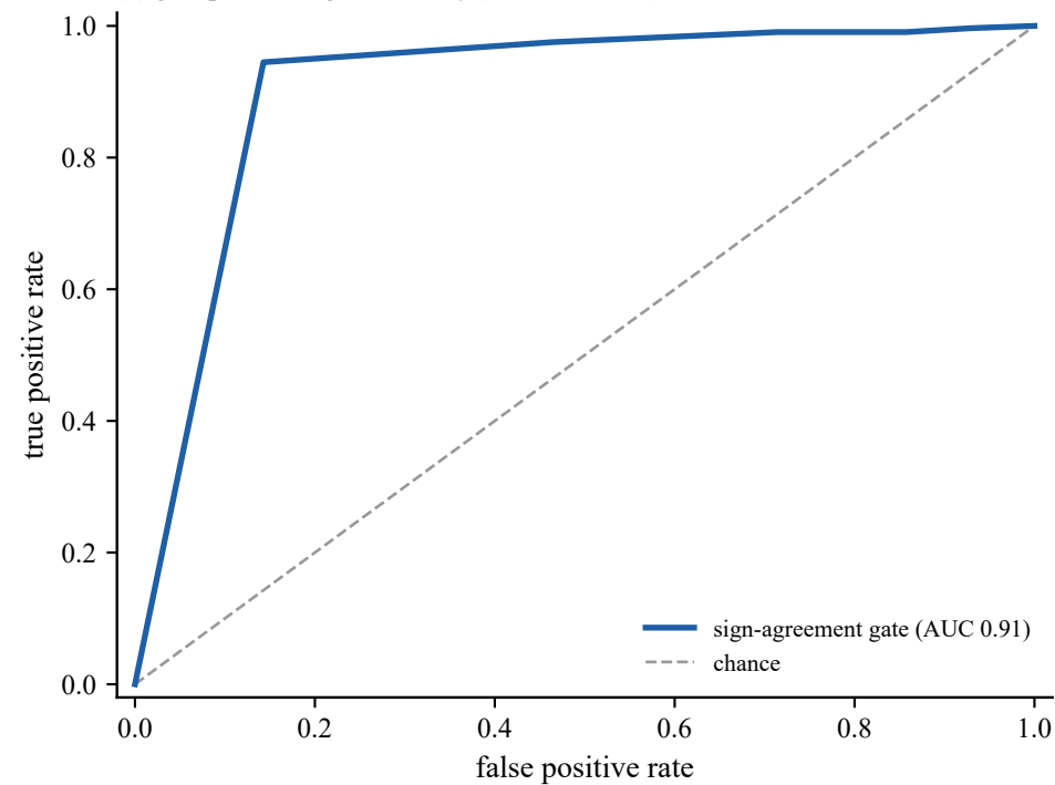
(a) gate predicts sign-reliability (external TMM)
